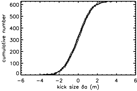
Figure 5. Distribution of kicks (changes in semi-major axis) felt by our simulated 100-m moonlet embedded in a ring with surface density \Sigma = 40 g cm ^{-2} , maximum particle size r_{\max} = 10 m, minimum particle size r_{\min} = 2.5 m, and power-law index q = 3 for the differential size distribution of particles. Kicks are computed every time interval \Omega^{-1} ; their cumulative distribution (solid line) conforms closely to a Gaussian (open circles). The typical kick size, \delta a \sim 1.5 m, is consistent with our order-of-magnitude estimate in Eq. 18.
