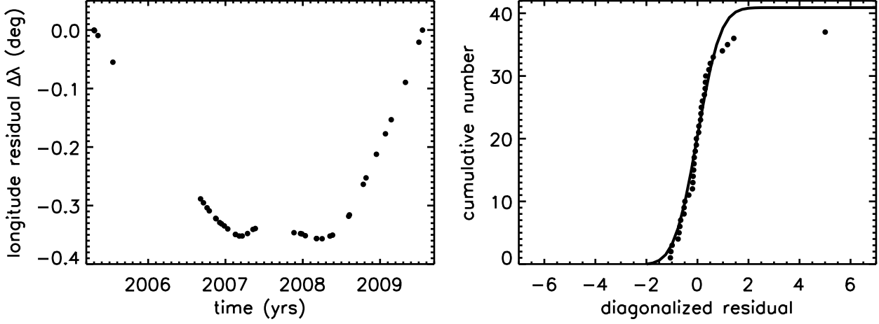
Figure 2. Checking the diagonalization test with a simulated integrated Gaussian random walk. A kick of 1 m in semi-major axis is applied every \delta t = \Omega^{-1} = 8842 s. The left panel shows the simulated longitude residuals sampled at the Blériot observation times (binned). For display purposes, we subtracted a linear trend to place the first and last data points at zero longitude residual. The right panel shows the results of the diagonalization test. The sorted diagonalized residuals (filled circles) are a reasonable match for Gaussian random variables (solid line). The 4 outliers dropped in calculating \hat{c} all lie outside the range shown in this plot.
