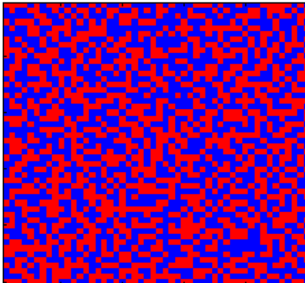
FIGURE 2. Signs of the i.i.d. Gaussian field on the 50 \times 50 discrete torus
