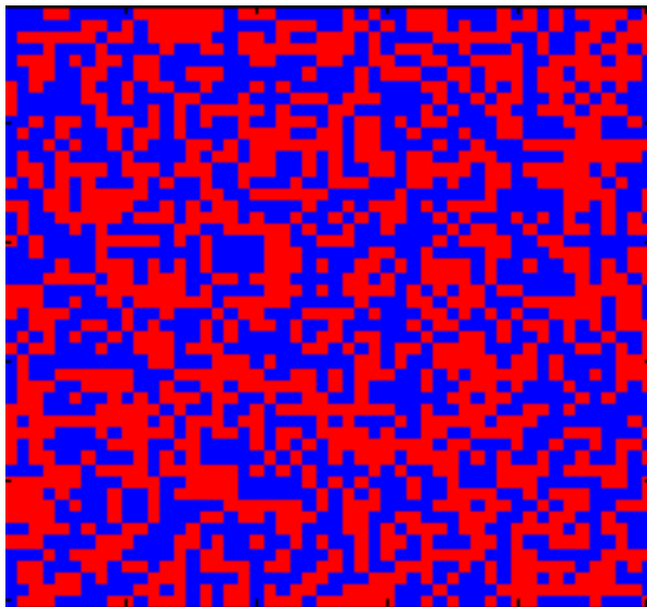
FIGURE 1. Signs of the Gaussian field arising from the simple random walk on the 50 \times 50 discrete torus
