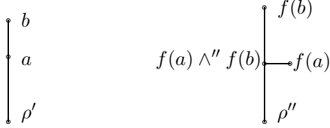
FIGURE 3 illustrates the shapes of the trees spanned by \{\rho', a, b\} and by \{\rho'', f(a), f(b)\} . The point f(a) lies somewhere on the arc [\rho'', f(b)] .
