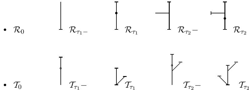
FIGURE 1 illustrates how the tree-valued processes (\mathcal{R}_t; t \geq 0) and (\mathcal{T}_t; t \geq 0) evolve. (The bold dots re-present an edge of length zero, while the small dots indicate the position of the cut point that is going to show up at the next moment.)
