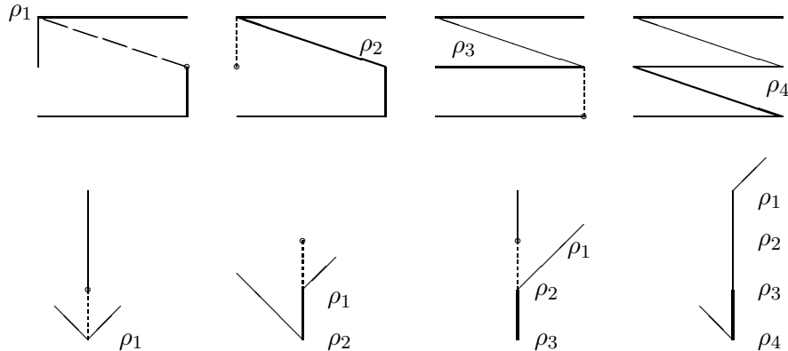
FIGURE 4 illustrates Aldous-Broder algorithm in discrete time. Here the dots mark the vertices that become the root in the next step. Once the new root is chosen we erase the edge adjacent to the new root on the path from the old to the new root and insert an edge connecting the old to the new root. The bold edges in the picture present the edges introduced recently.
