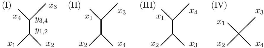
FIGURE 2 shows the 4 different shapes of a labeled tree with 4 leaves.
